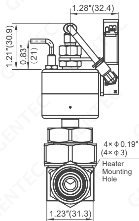
with Heater Mounting Hole (standard, normally closed)
