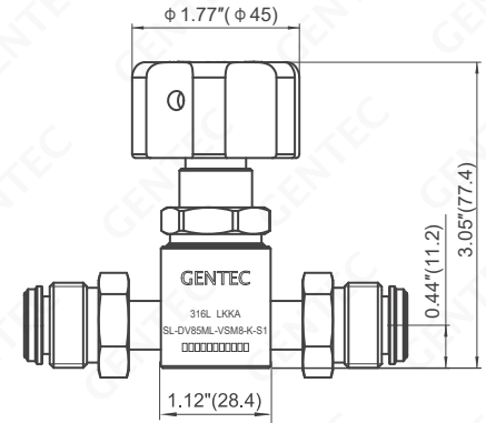
Handwheel (With Display)
